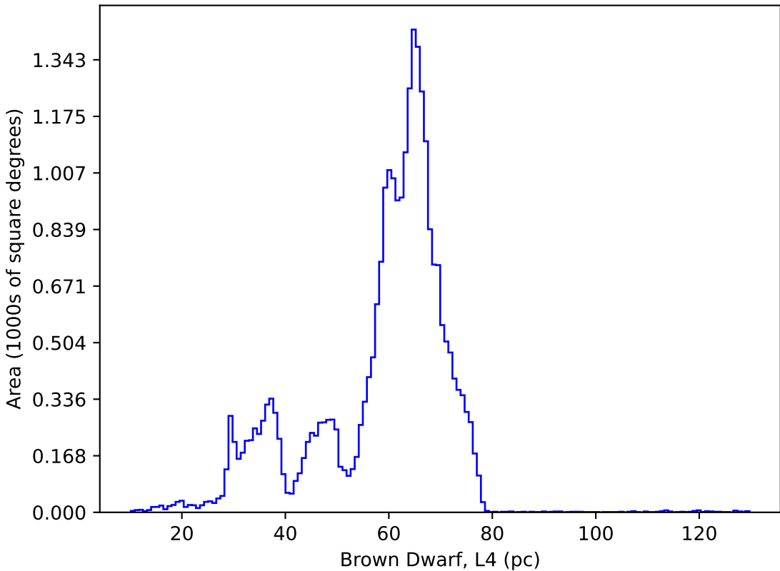
roman_v3.3_10yrs : Brown Dwarf, L4
