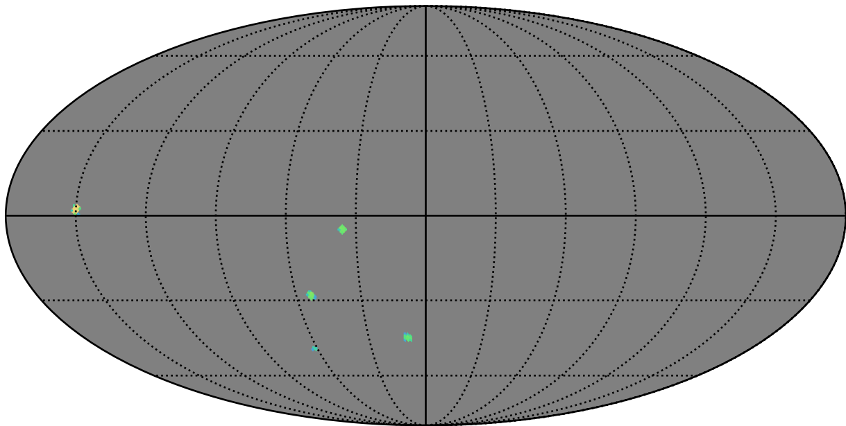
roman_v3.3_10yrs z band: AGN_TimeLag_5_days
