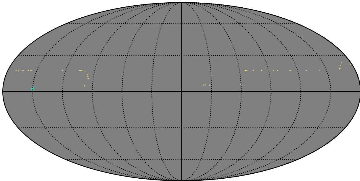
roman_v3.3_10yrs y band: AGN_TimeLag_5_days
