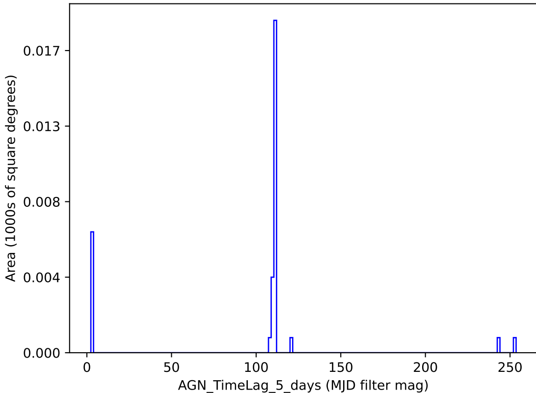
roman_v3.3_10yrs y band: AGN_TimeLag_5_days
