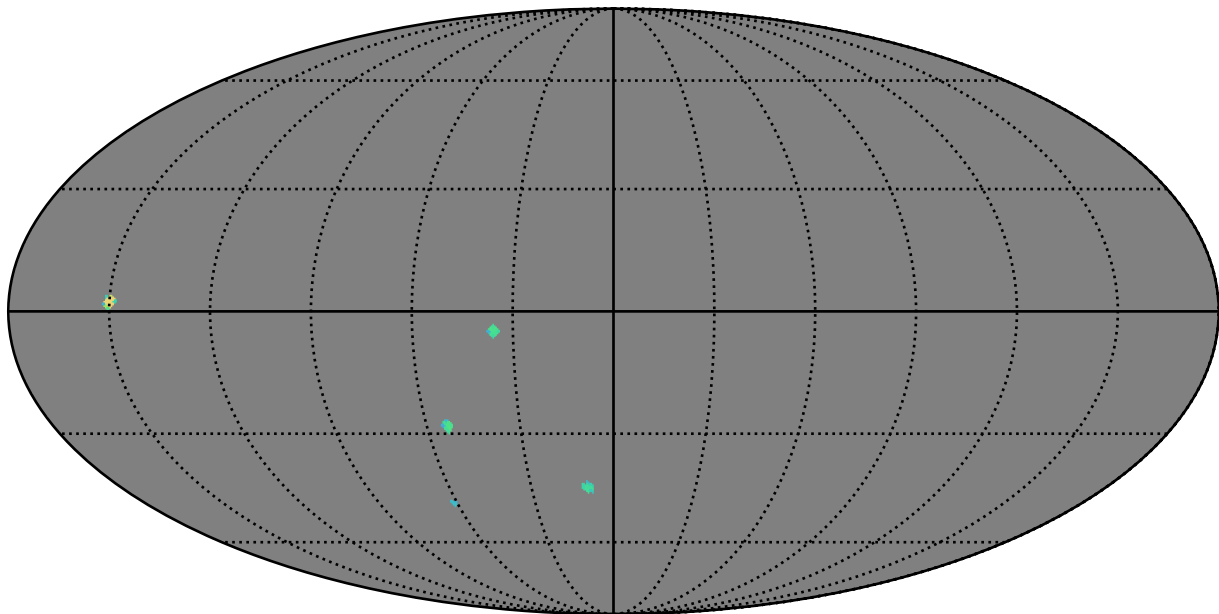
roman_v3.3_10yrs r band: AGN_TimeLag_5_days
