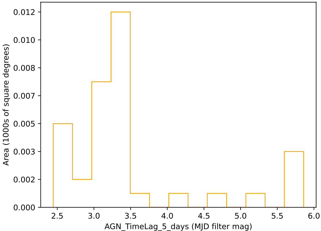
roman_v3.3_10yrs r band: AGN_TimeLag_5_days
