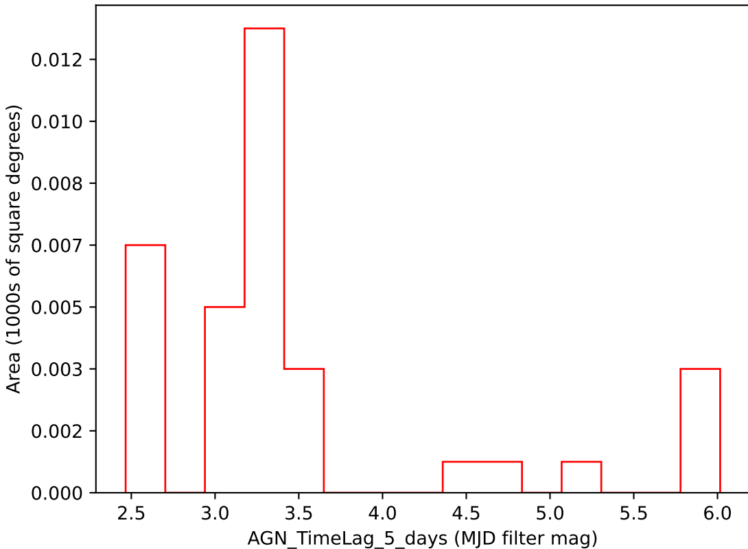
roman_v3.3_10yrs i band: AGN_TimeLag_5_days
