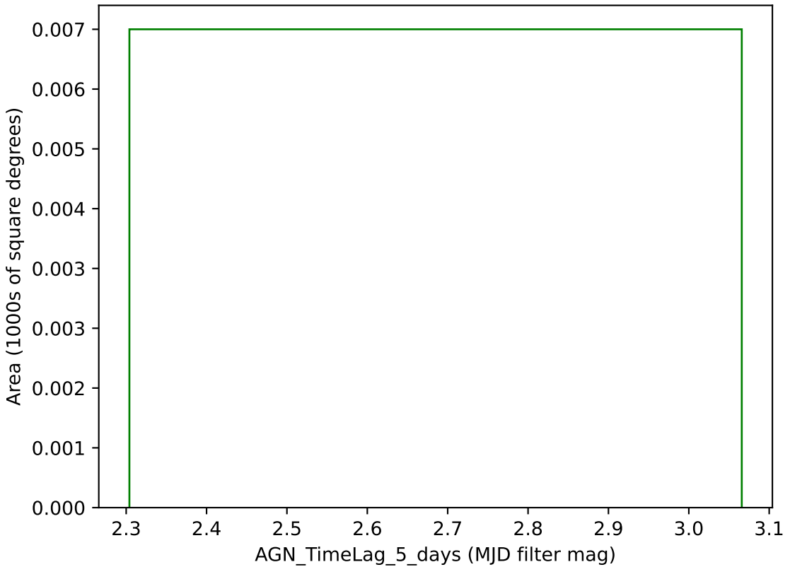
roman_v3.3_10yrs g band: AGN_TimeLag_5_days
