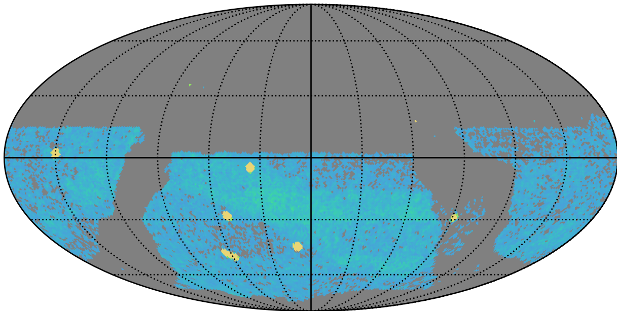
roman_v3.3_10yrs z band: AGN_TimeLag_100_days
