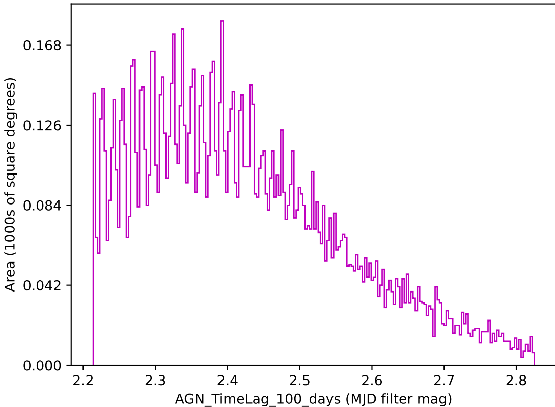
roman_v3.3_10yrs z band: AGN_TimeLag_100_days
