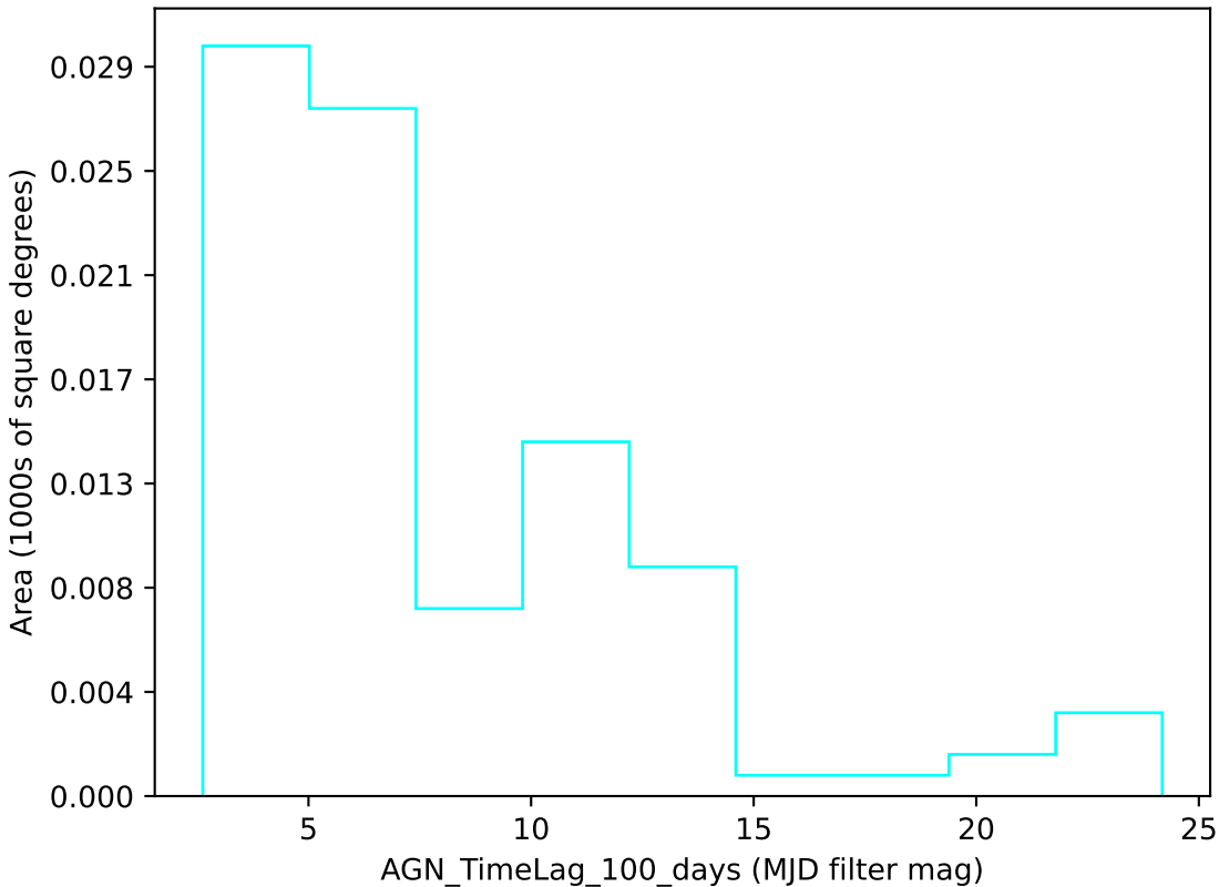
roman_v3.3_10yrs u band: AGN_TimeLag_100_days
