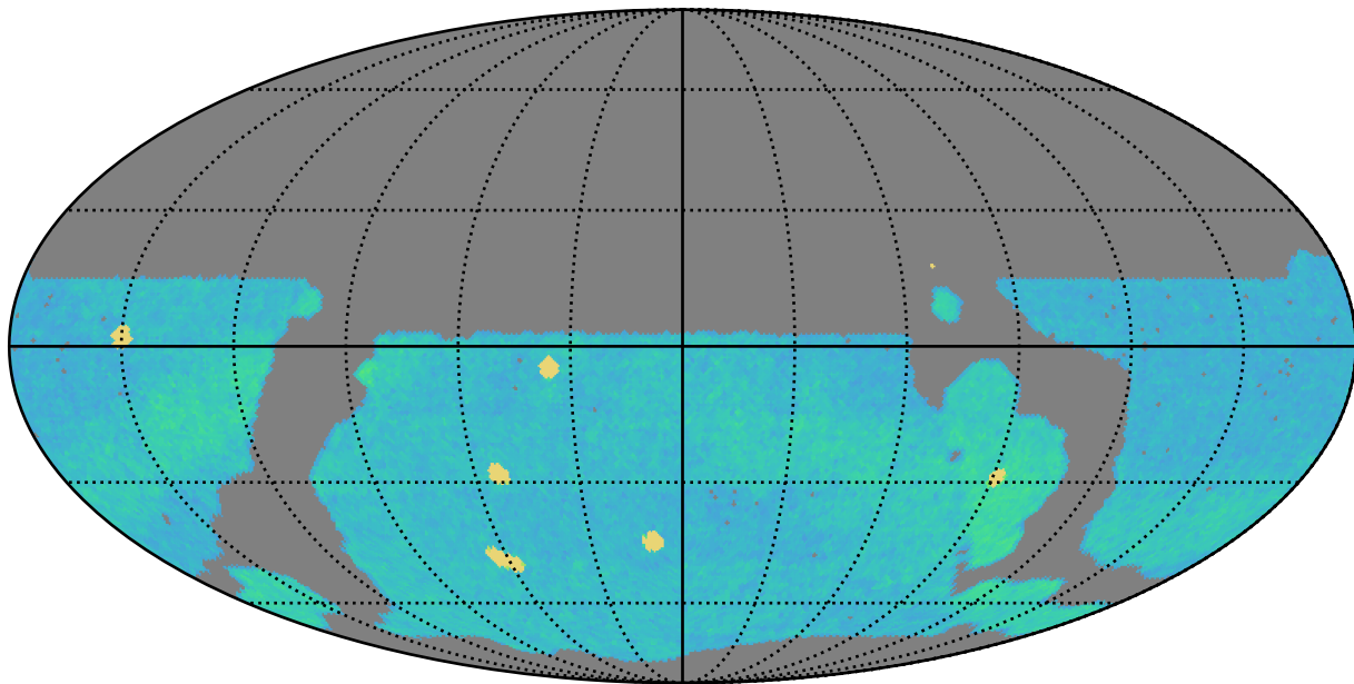
roman_v3.3_10yrs r band: AGN_TimeLag_100_days
