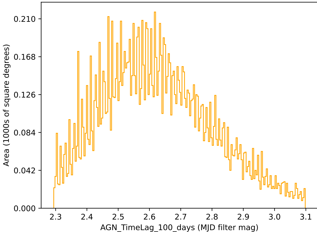
roman_v3.3_10yrs r band: AGN_TimeLag_100_days
