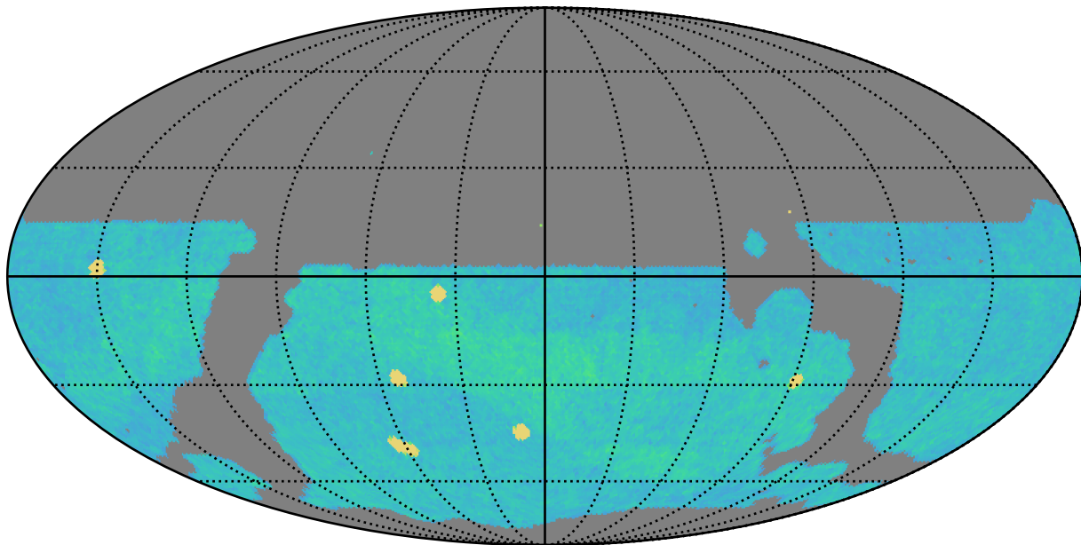
roman_v3.3_10yrs i band: AGN_TimeLag_100_days
