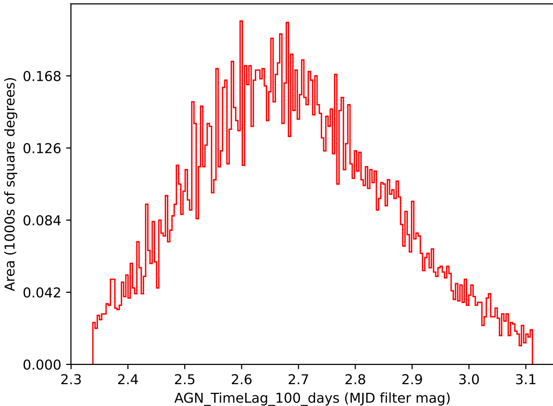
roman_v3.3_10yrs i band: AGN_TimeLag_100_days
