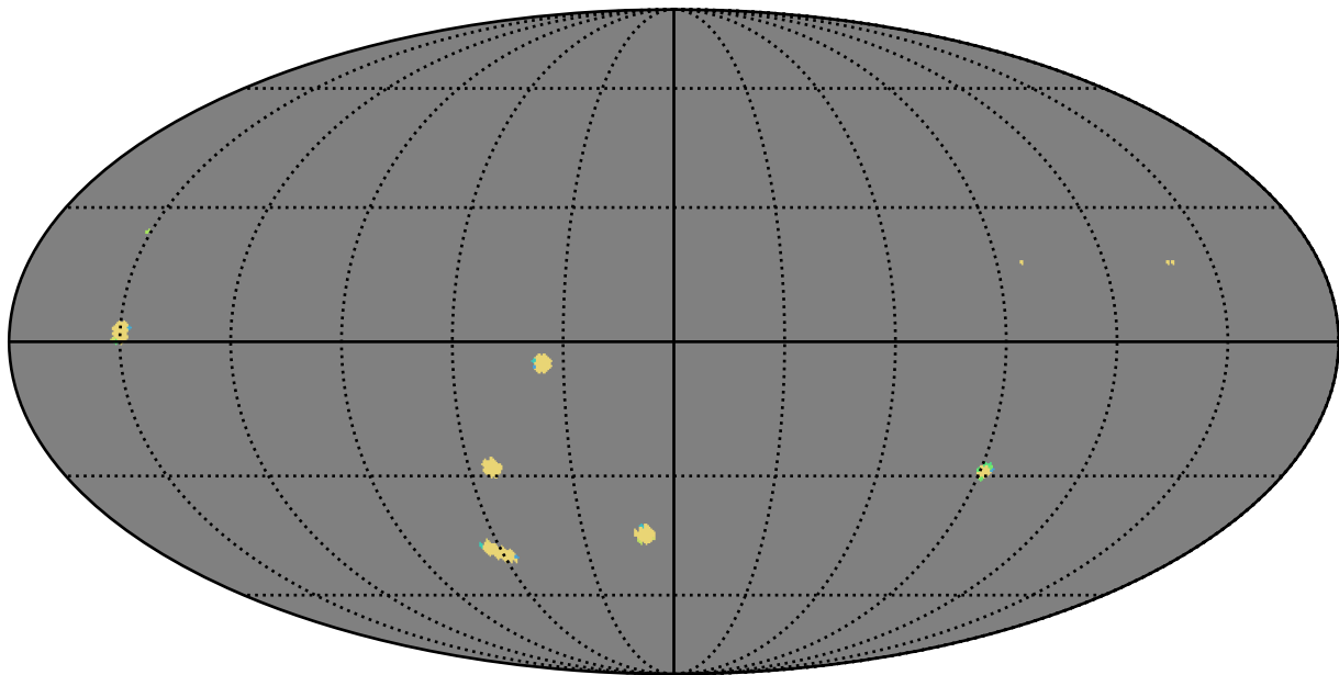
roman_v3.3_10yrs g band: AGN_TimeLag_100_days
