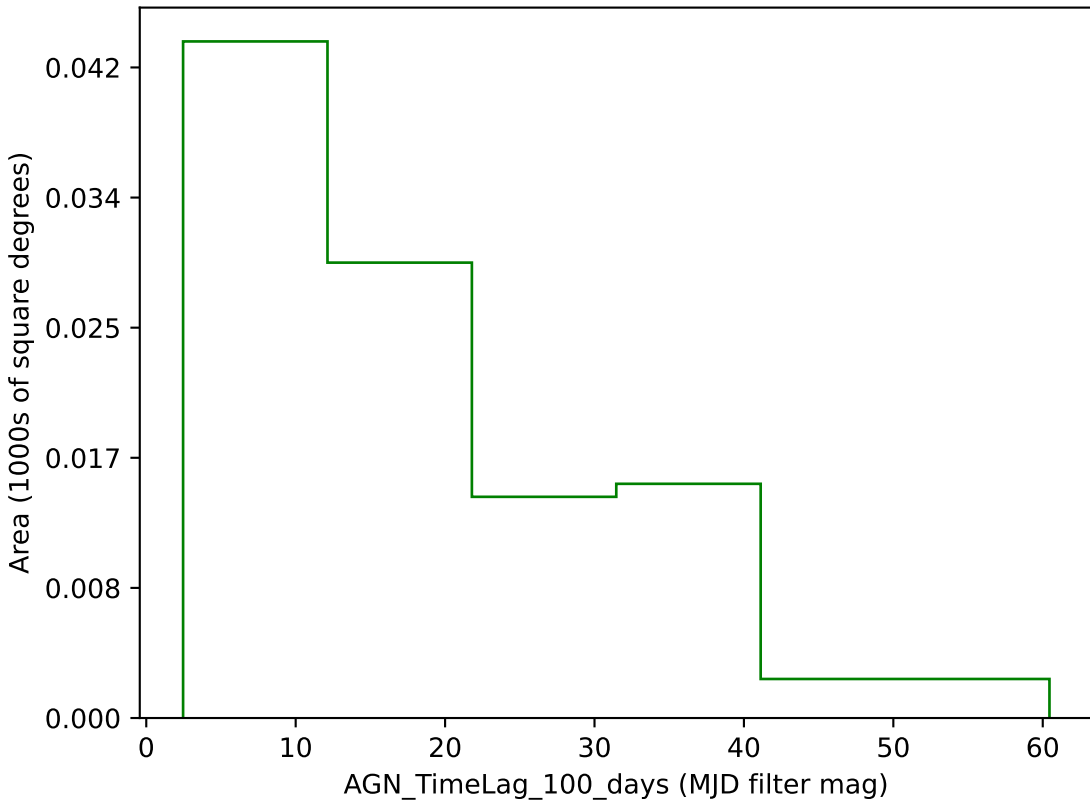
roman_v3.3_10yrs g band: AGN_TimeLag_100_days
