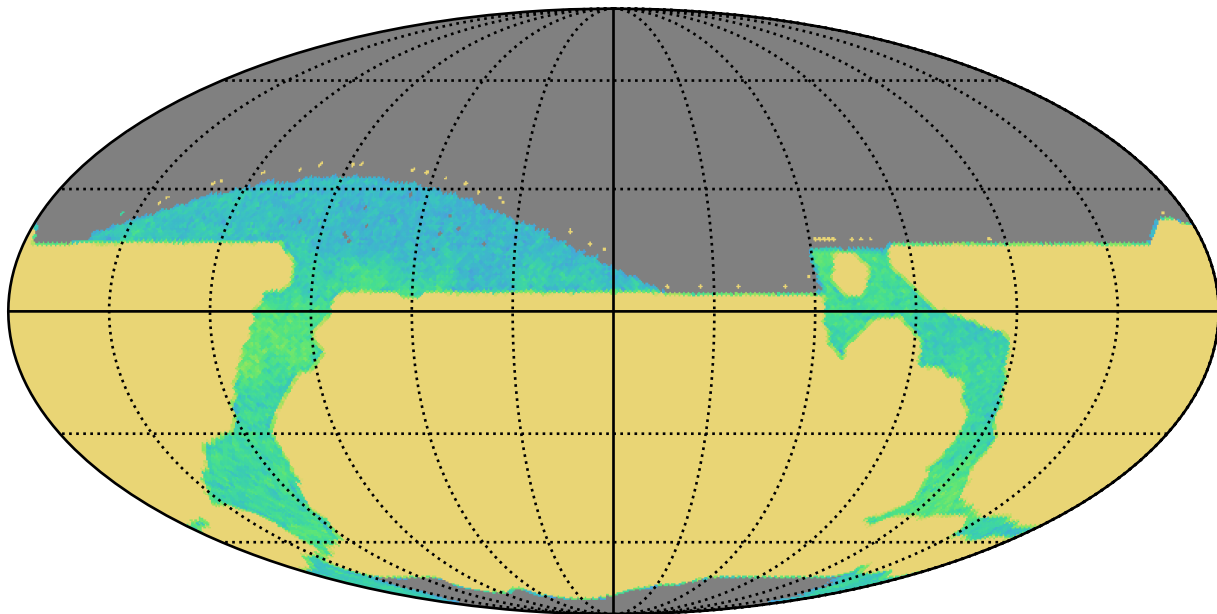
roman_v3.3_10yrs all bands: AGN_TimeLag_100_days
