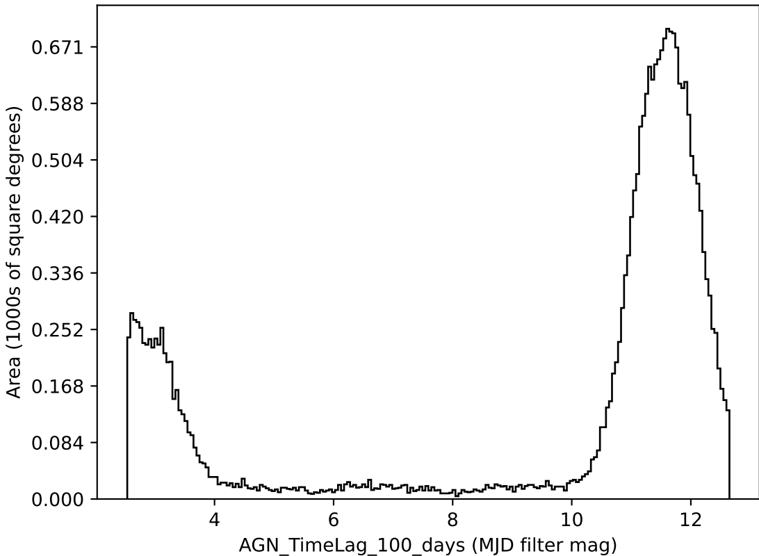
roman_v3.3_10yrs all bands: AGN_TimeLag_100_days
