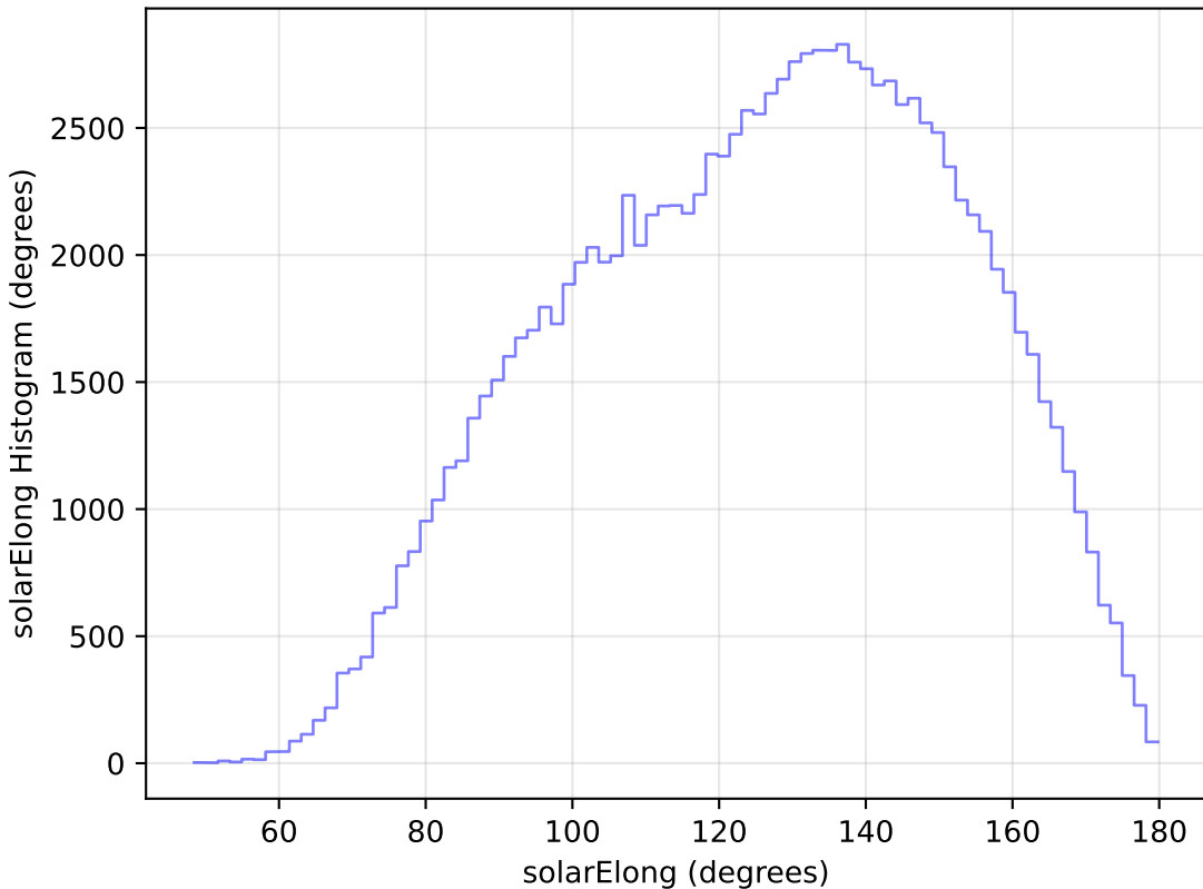
roman_v3.3_10yrs WFD u band: solarElong Histogram
