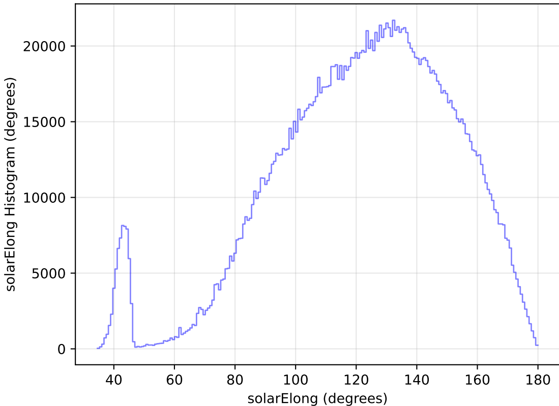
roman_v3.3_10yrs WFD all bands: solarElong Histogram
