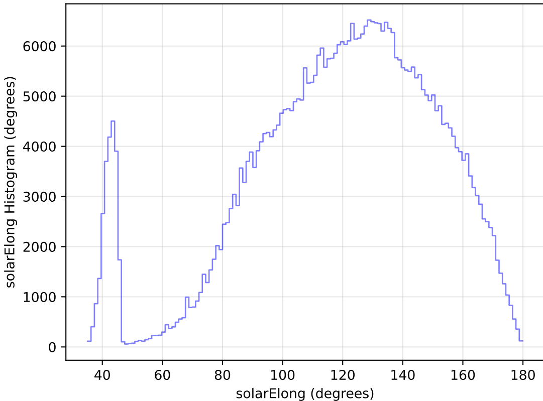
roman_v3.3_10yrs All sky z band: solarElong Histogram
