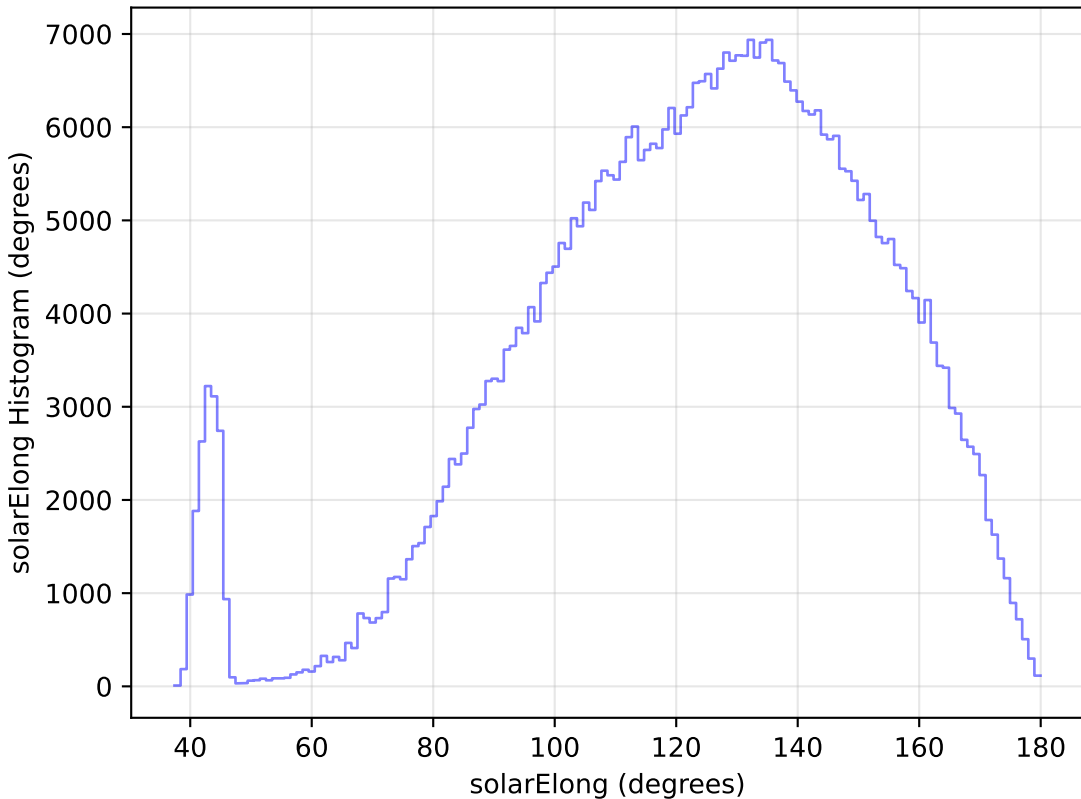
roman_v3.3_10yrs All sky r band: solarElong Histogram
