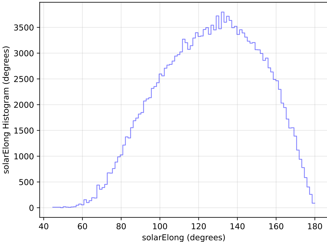
roman_v3.3_10yrs All sky g band: solarElong Histogram
