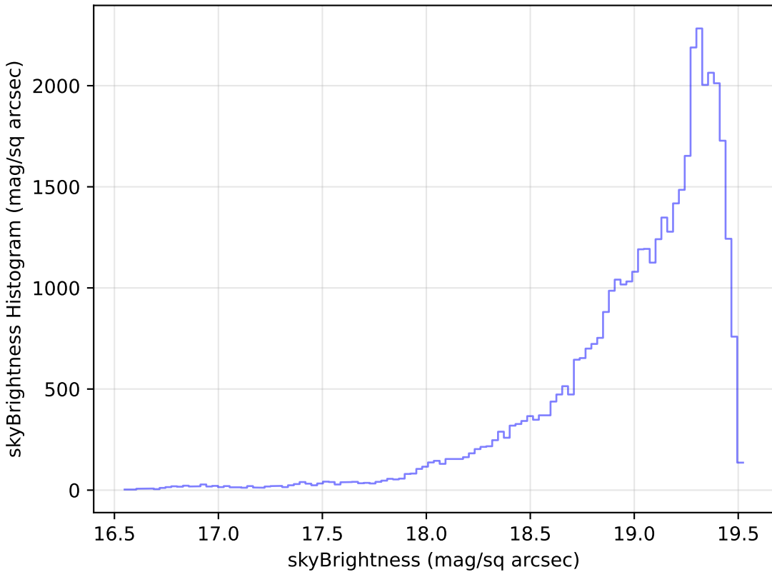
roman_v3.3_10yrs Yr 1 z band: skyBrightness Histogram
