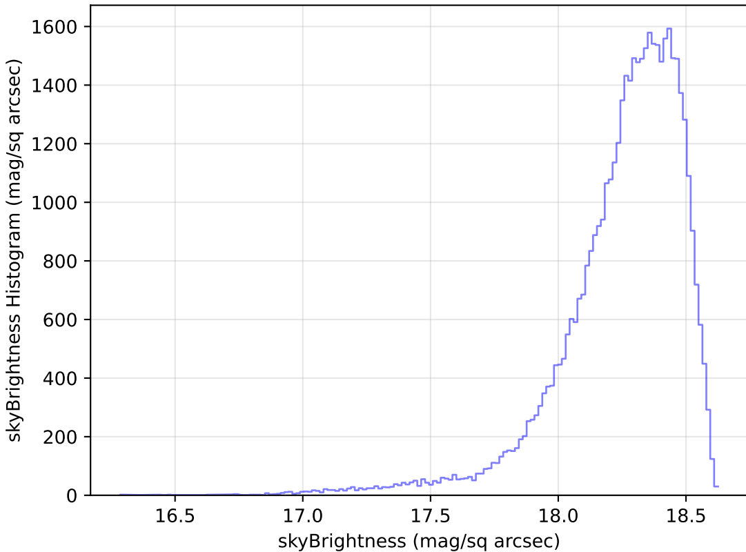
roman_v3.3_10yrs Yr 1 y band: skyBrightness Histogram
