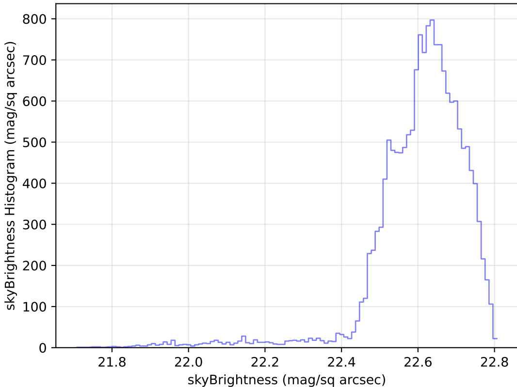
roman_v3.3_10yrs Yr 1 u band: skyBrightness Histogram
