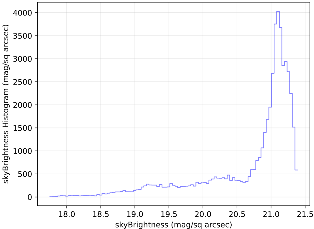
roman_v3.3_10yrs Yr 1 r band: skyBrightness Histogram
