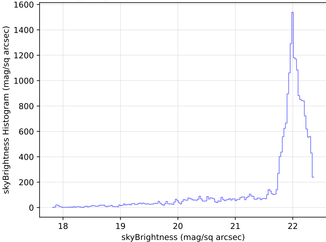
roman_v3.3_10yrs Yr 1 g band: skyBrightness Histogram
