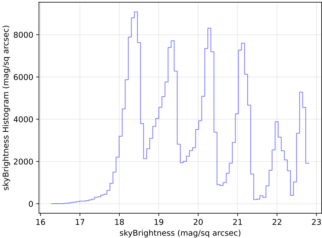
roman_v3.3_10yrs Yr 1 all bands: skyBrightness Histogram
