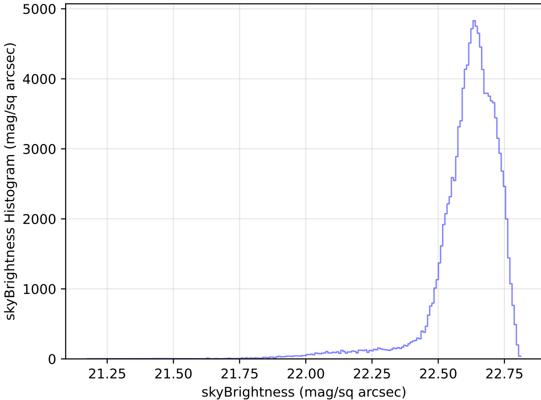
roman_v3.3_10yrs WFD u band: skyBrightness Histogram
