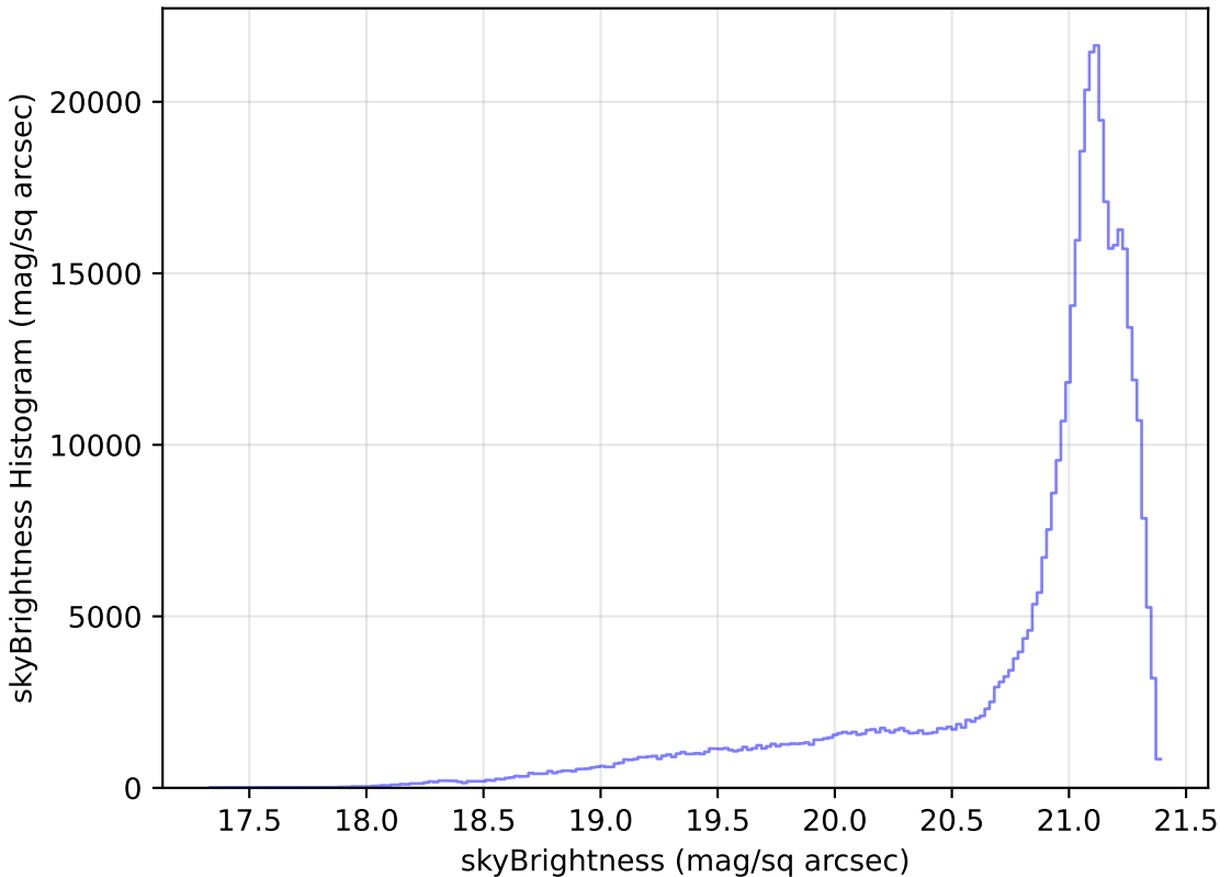
roman_v3.3_10yrs WFD r band: skyBrightness Histogram
