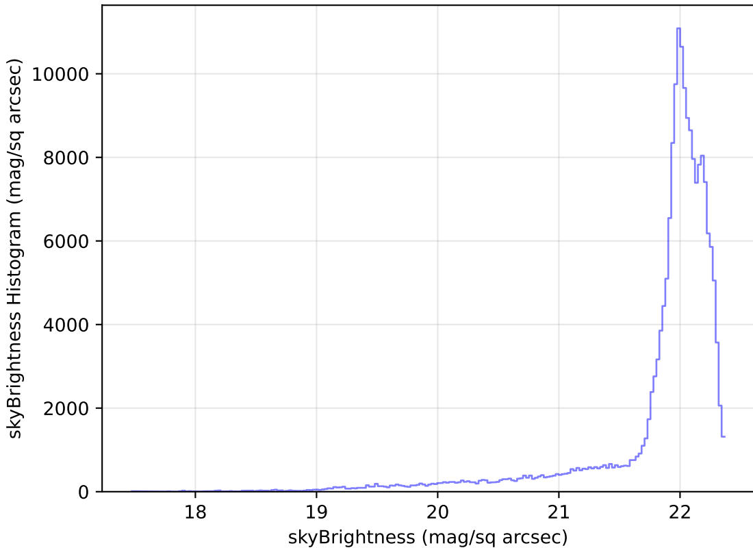
roman_v3.3_10yrs WFD g band: skyBrightness Histogram
