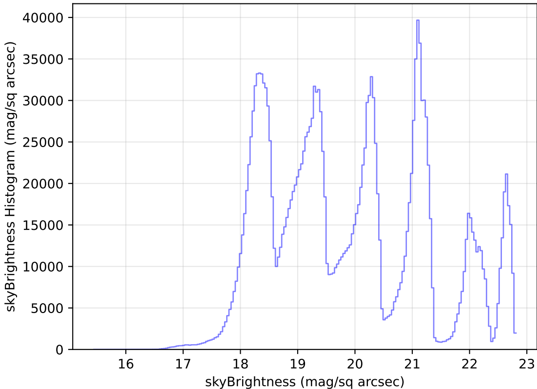
roman_v3.3_10yrs WFD all bands: skyBrightness Histogram
