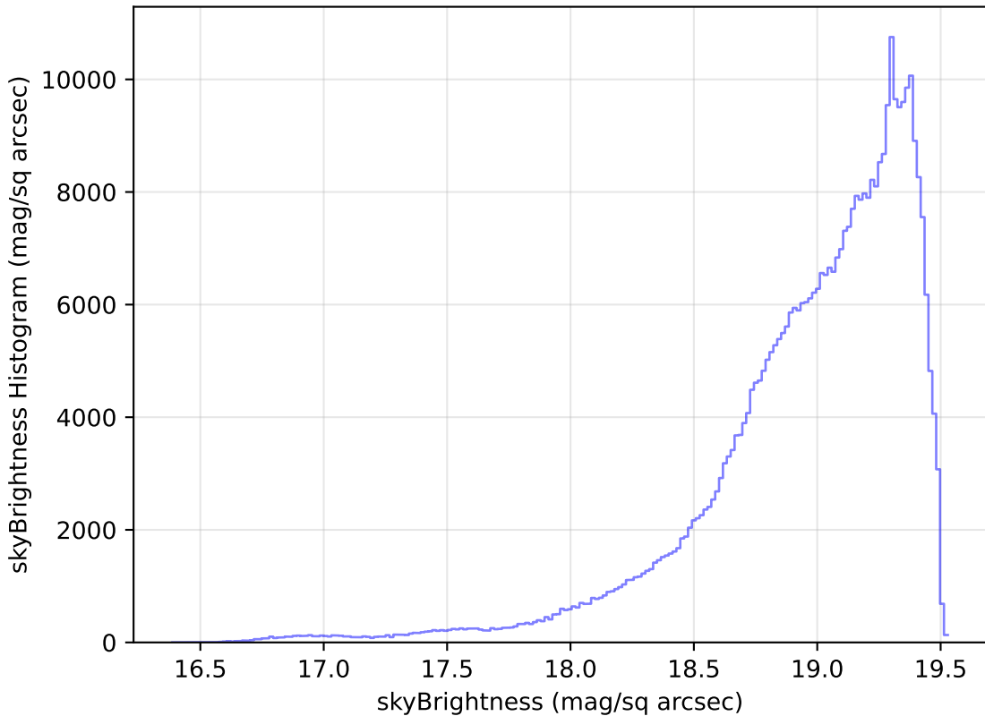
roman_v3.3_10yrs All sky z band: skyBrightness Histogram
