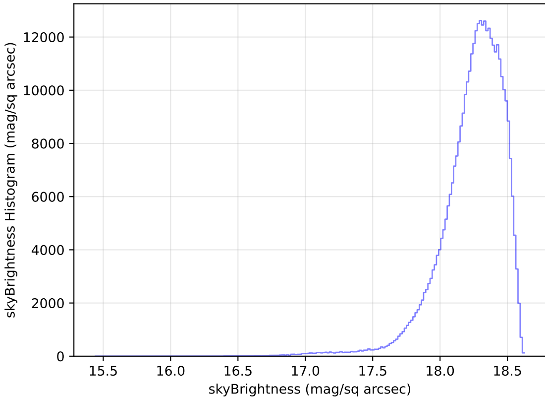
roman_v3.3_10yrs All sky y band: skyBrightness Histogram
