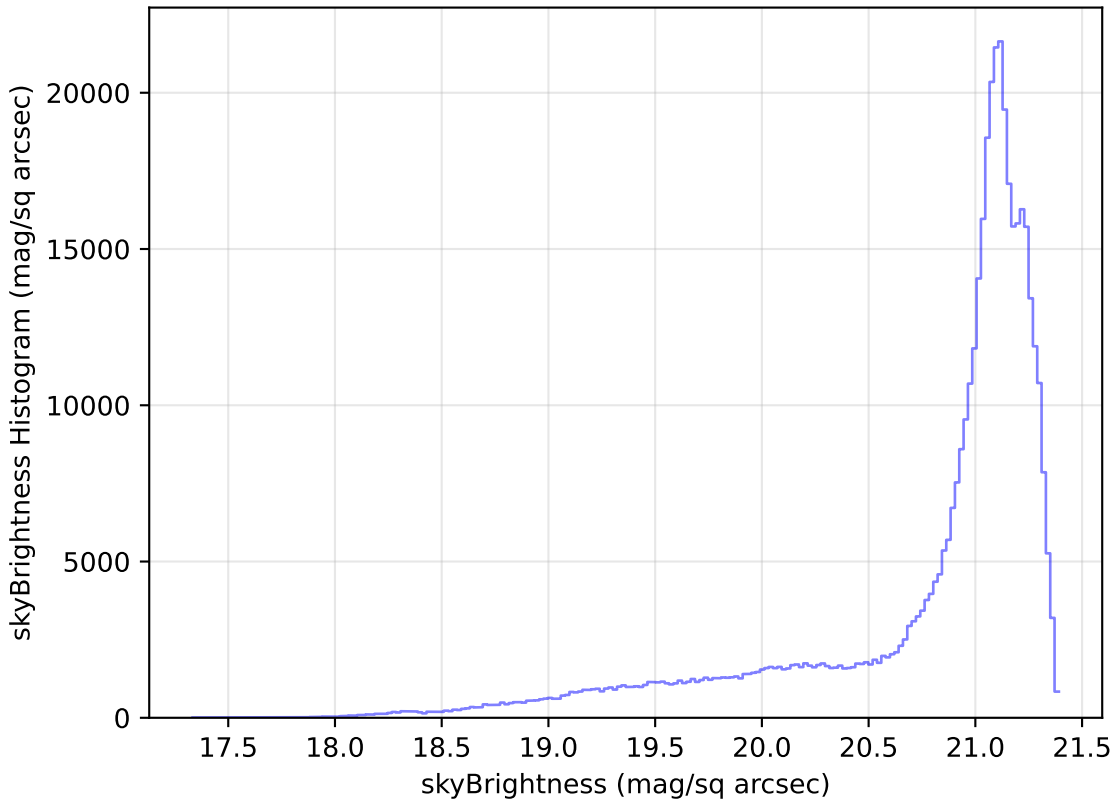
roman_v3.3_10yrs All sky r band: skyBrightness Histogram
