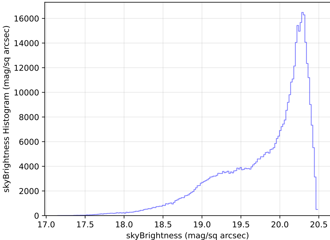
roman_v3.3_10yrs All sky i band: skyBrightness Histogram
