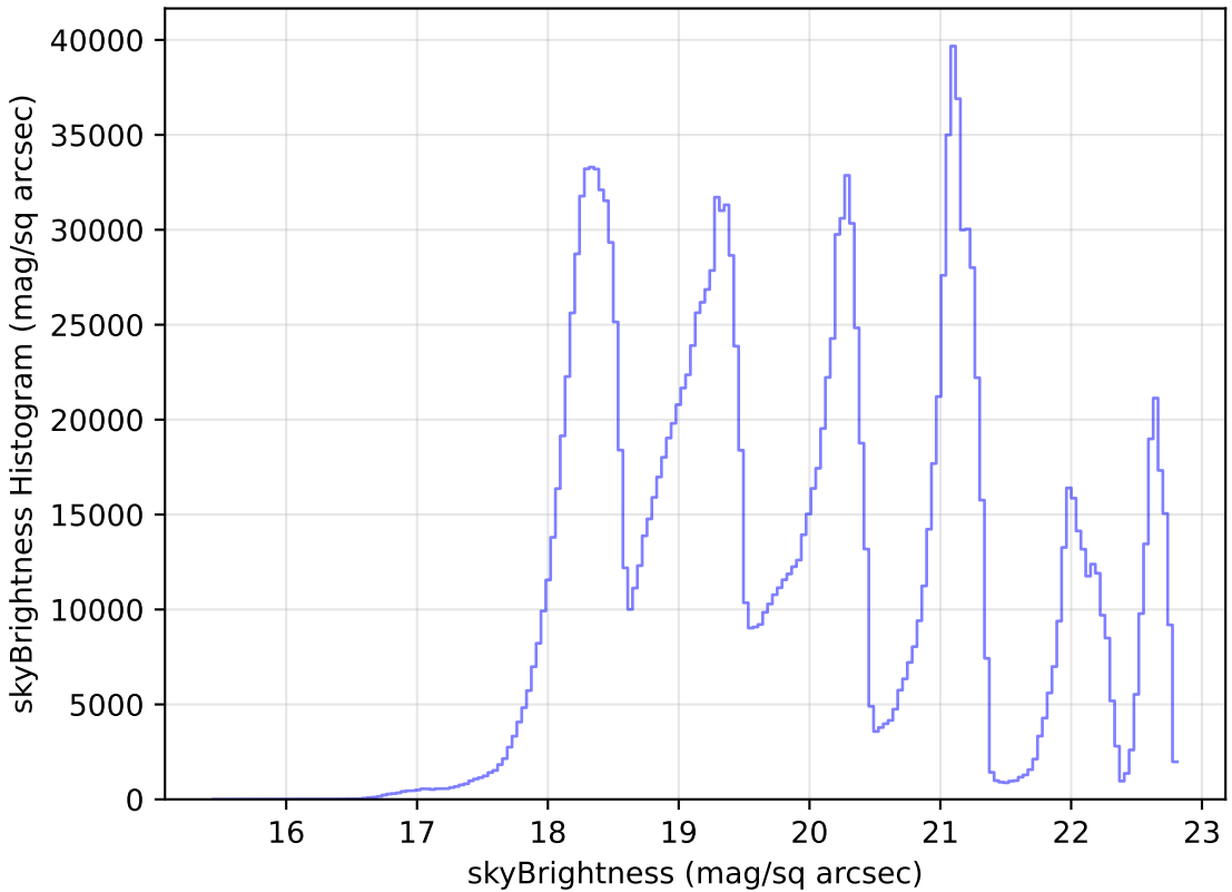
roman_v3.3_10yrs All sky all bands: skyBrightness Histogram
