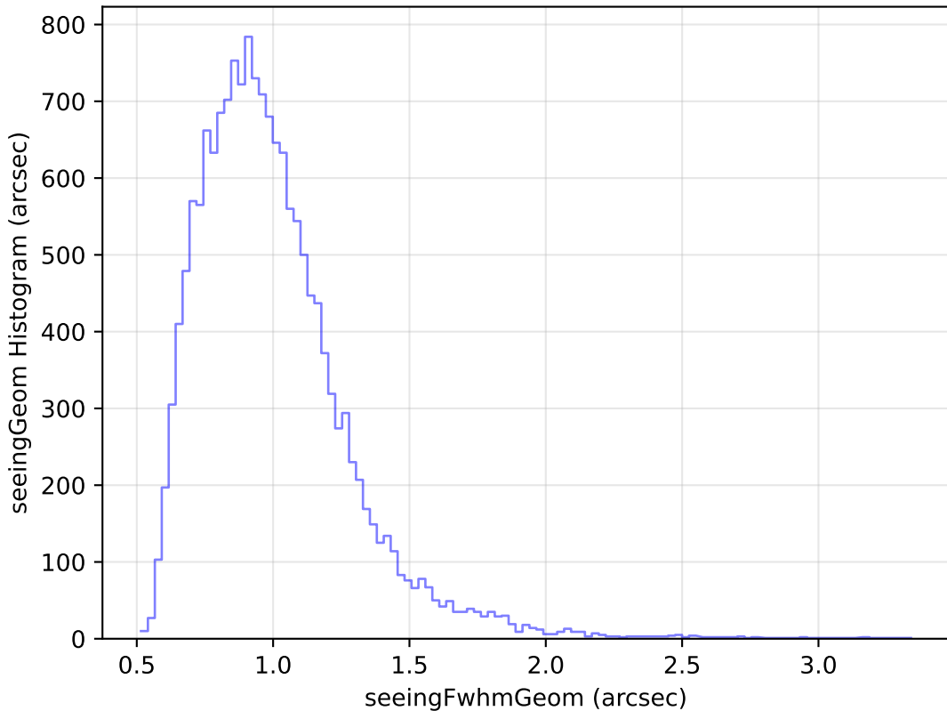
roman_v3.3_10yrs Yr 1 u band: seeingGeom Histogram
