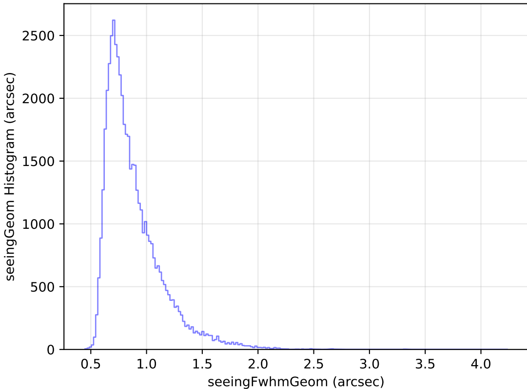
roman_v3.3_10yrs Yr 1 r band: seeingGeom Histogram
