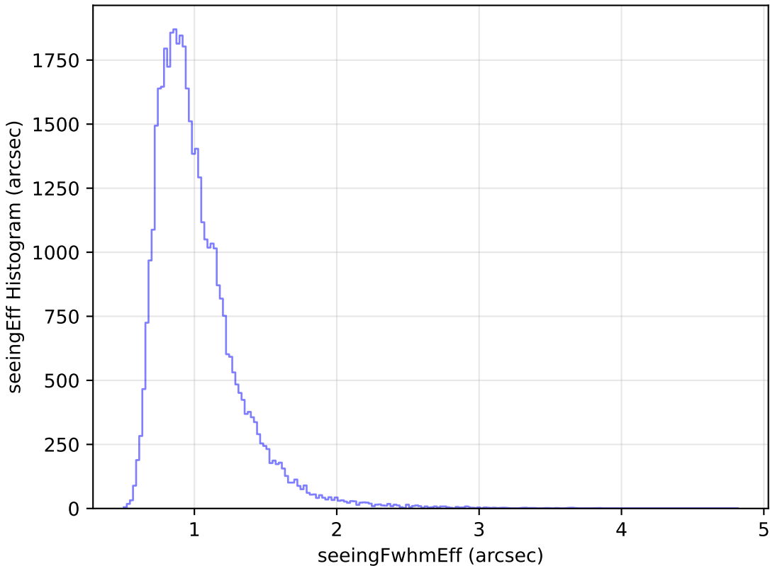
roman_v3.3_10yrs Yr 1 z band: seeingEff Histogram
