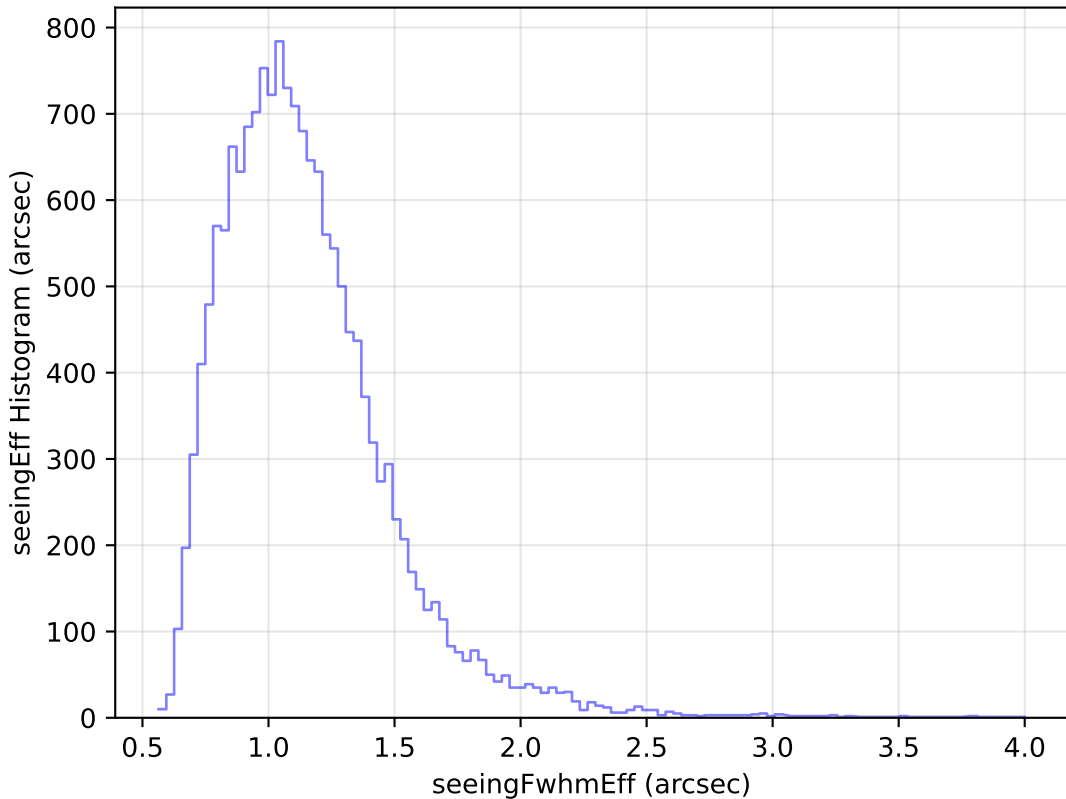
roman_v3.3_10yrs Yr 1 u band: seeingEff Histogram
