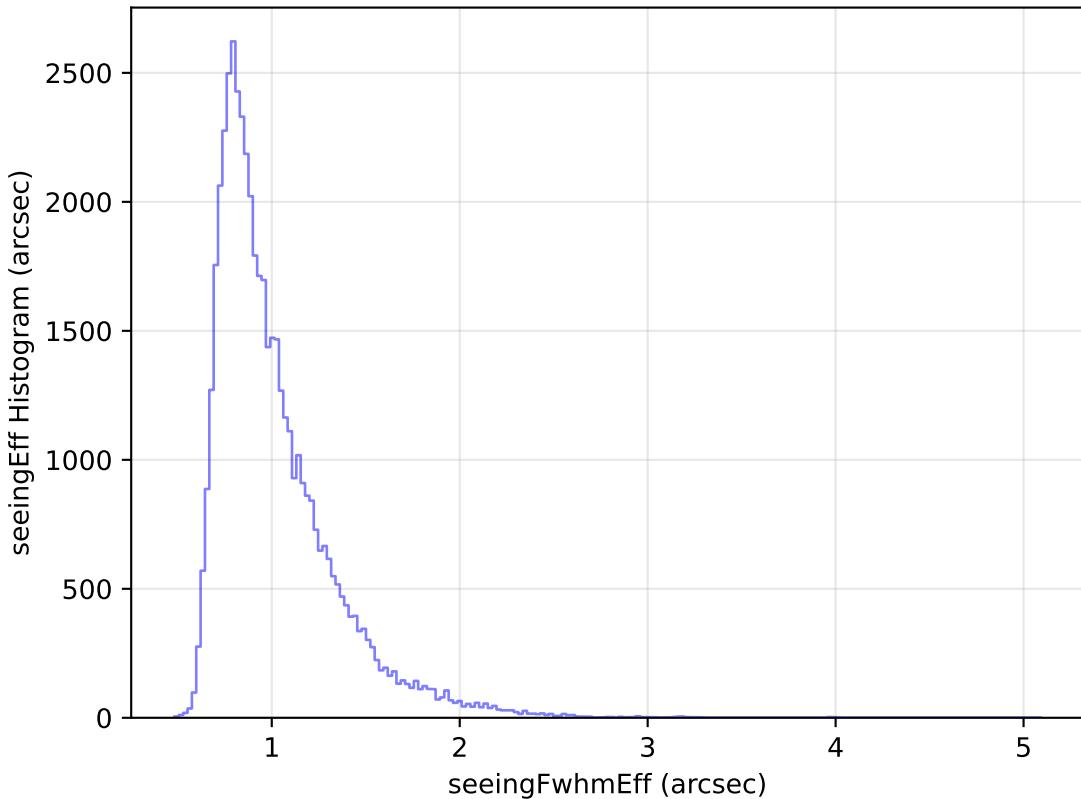
roman_v3.3_10yrs Yr 1 r band: seeingEff Histogram
