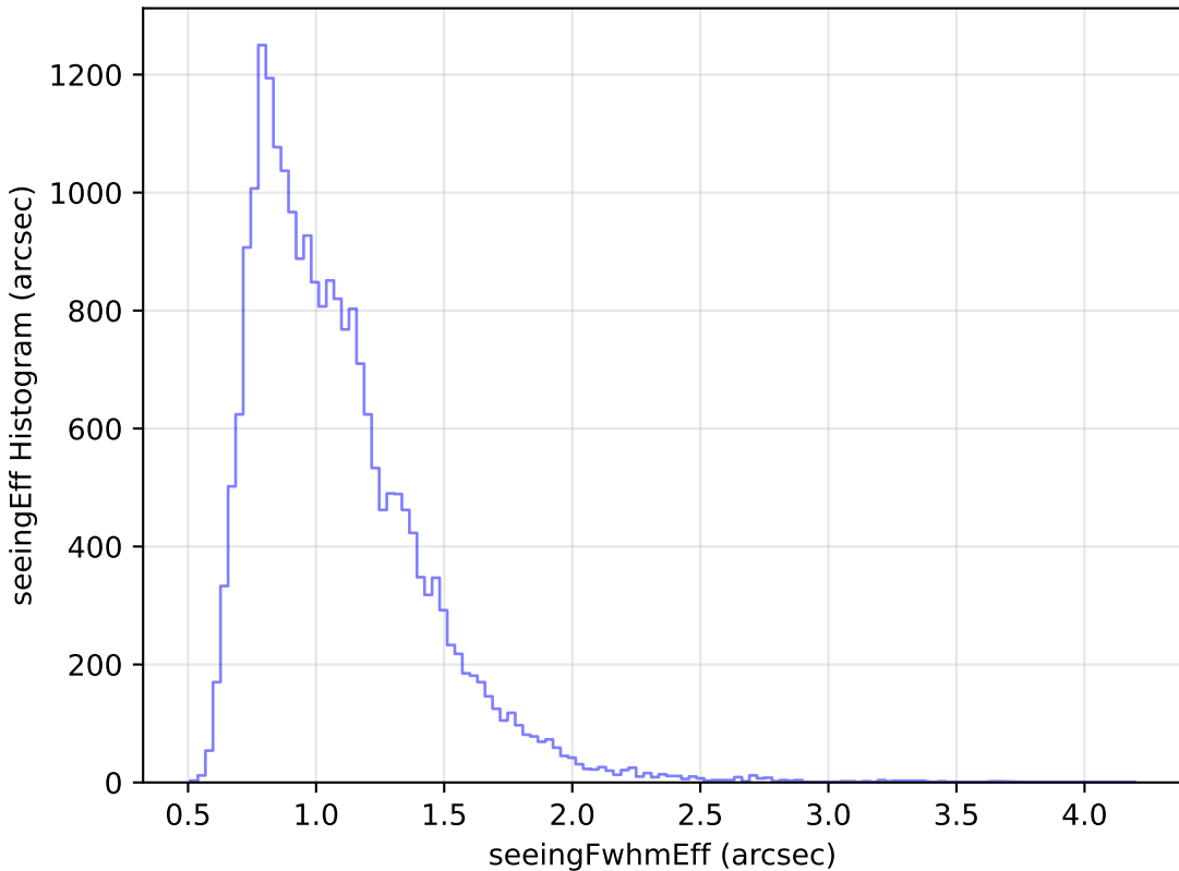
roman_v3.3_10yrs Yr 1 g band: seeingEff Histogram
