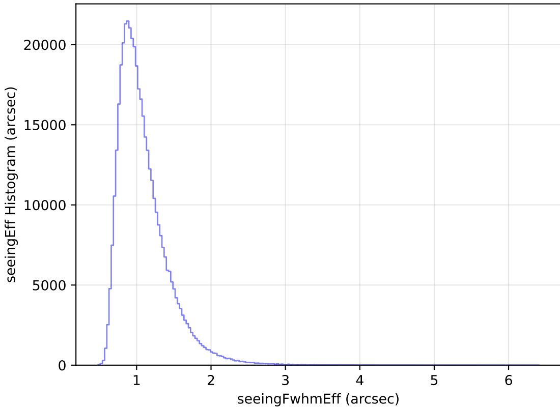
roman_v3.3_10yrs WFD z band: seeingEff Histogram
