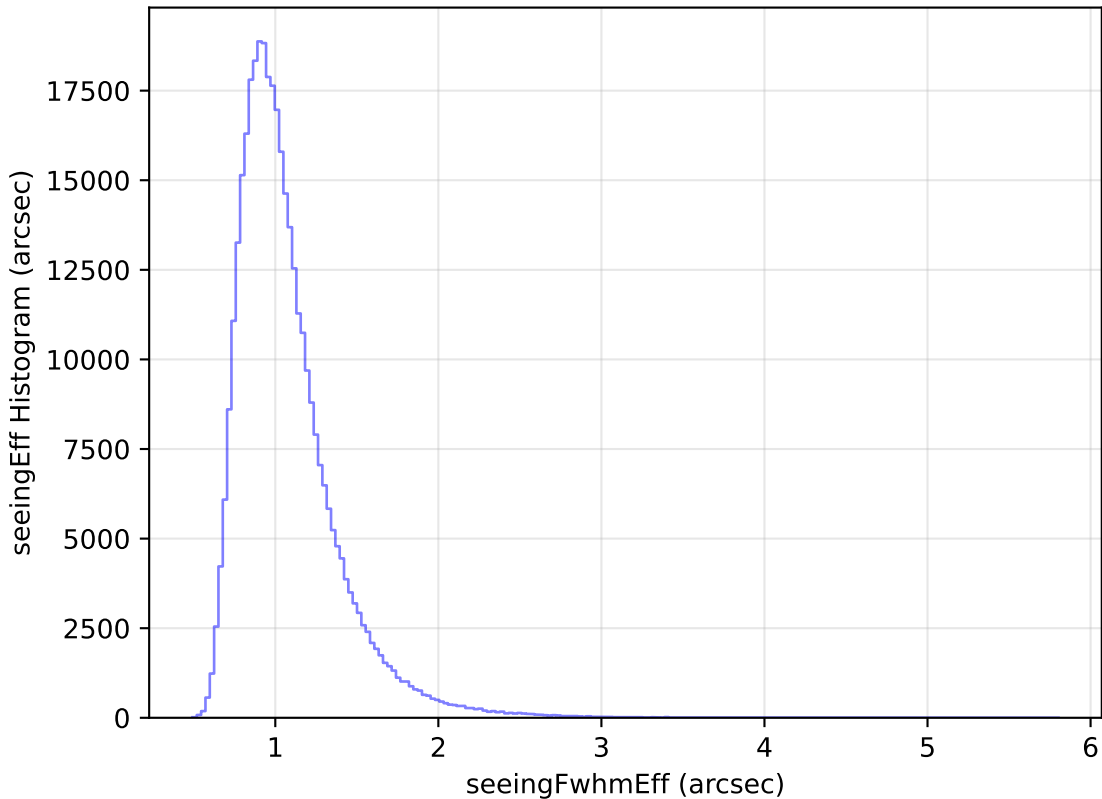
roman_v3.3_10yrs WFD y band: seeingEff Histogram
