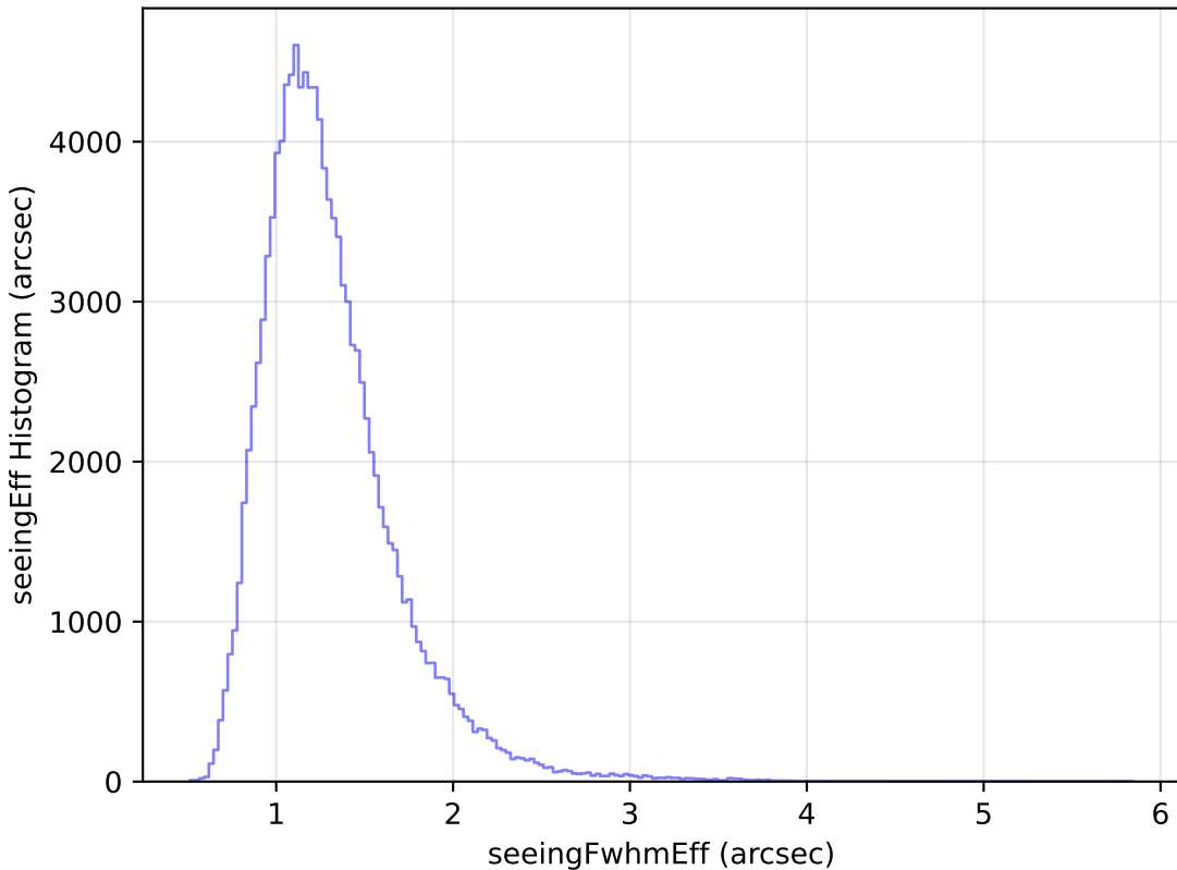
roman_v3.3_10yrs WFD u band: seeingEff Histogram
