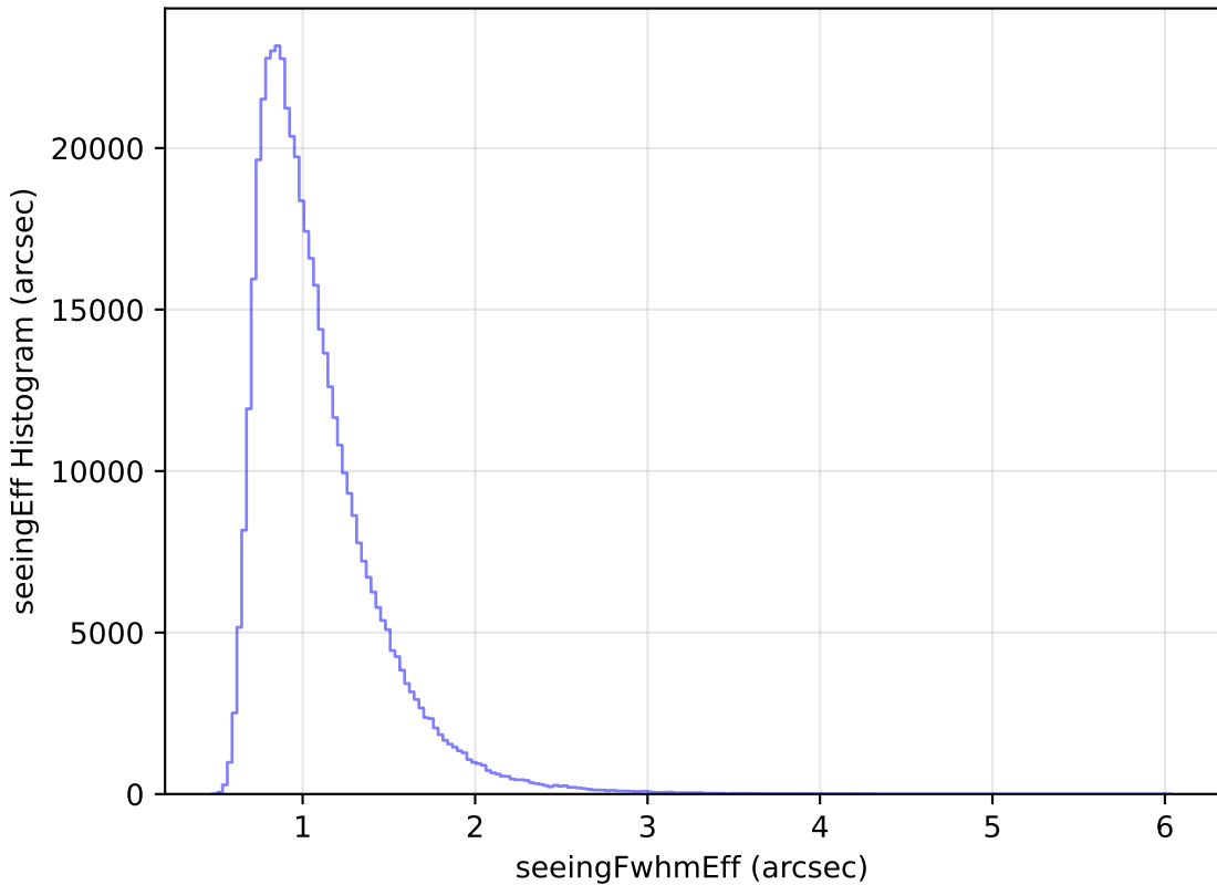
roman_v3.3_10yrs WFD i band: seeingEff Histogram
