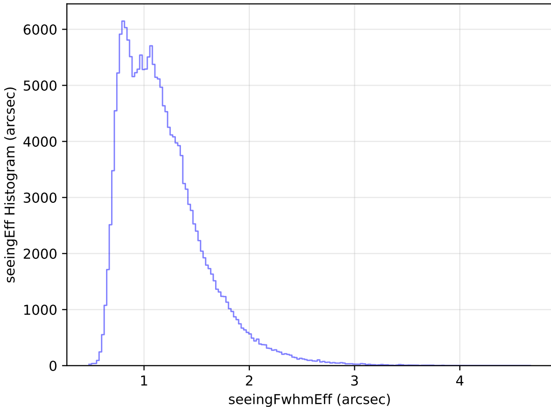
roman_v3.3_10yrs WFD g band: seeingEff Histogram
